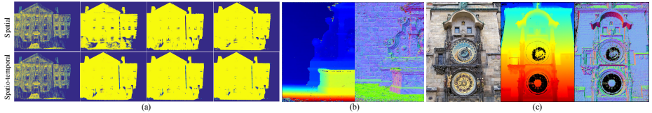
Fig. 5. (a) Comparison of spatial smoothness term [59] with our proposed spatial and temporal smoothness term for the occlusion variables Z . Algorithm starts from the left with the first sweep and is followed by consecutive sweeps to the right. (b) Estimated depths and normals using standard PatchMatch propagation ( cf. Fig. 3 for ours). (c) Reference image with filtered depths and normals for crowd-sourced images
