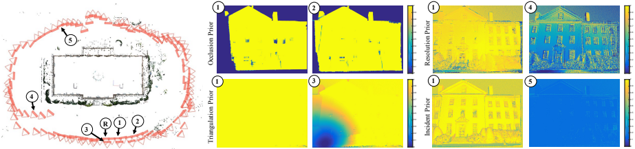
Fig. 4. Photometric and geometric priors for South Building dataset [20] between reference image (R) and each two selected source images (1-5).
