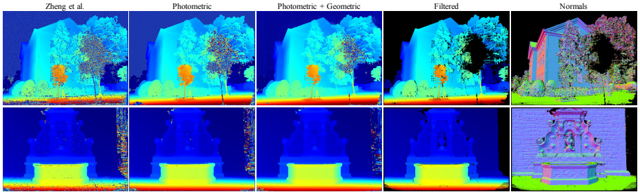
Fig. 3. Reconstruction results for South Building [20] and Fountain [48]. From left to right: Depth map by Zheng et al. [59], then ours only with the photometric term, with the photometric and geometric terms, and the final filtered depth and normal maps.
